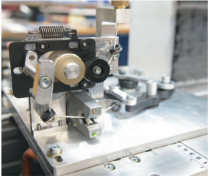
Yarn feed system with electronic yarn detection
